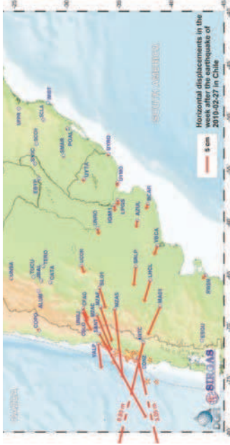
Figure 1: GPS station displacements after the Maule earthquake, Chile, 27 February 2010
