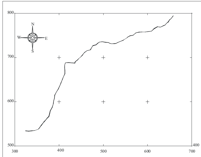
Figure 5: The horizontal section of the declivity at the height of 80m
