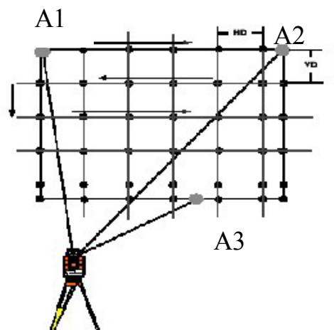
Figure 1: The definition of the surface to be swept.
