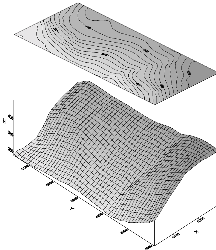
Figure 7: The 3d model generated by the map.
