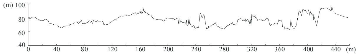
Figure 4: A longitudinal section of the declivity
