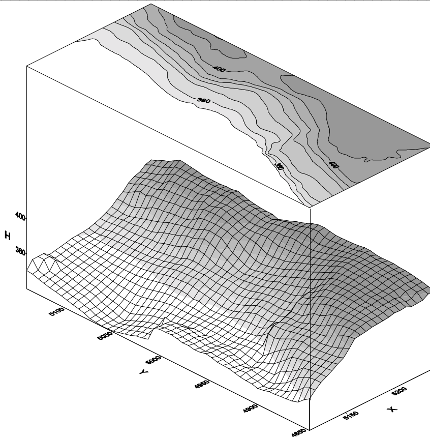
Figure 5: The 3d model created by using the measurements of the total station.
